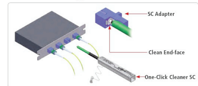
Illustration of cleaning procedure for SC connectors
